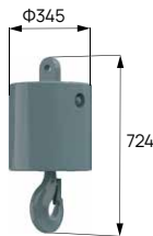
10t ball hook 球钩
